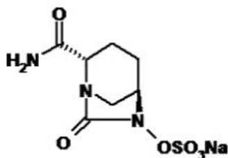
Figure 2 Chemical structure of avibactam sodium
